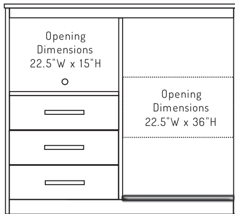
ABB-117 Micro-Fridge Combo Unit - NO Trim 48\"W x 22\"D x 43\"H
